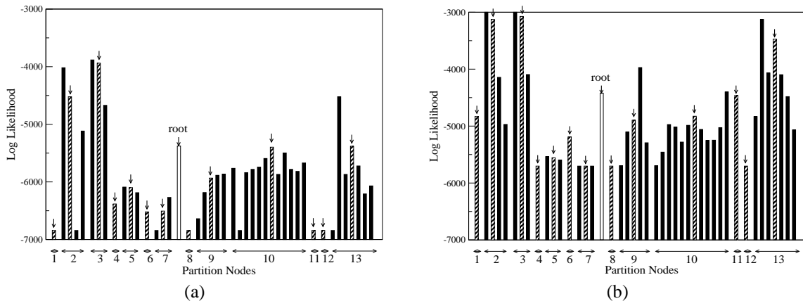
Figure 4. Likelihood values for the first three levels in the Washington Post partition tree for (a) Category News concept, and (b) Taxonomy News concept
